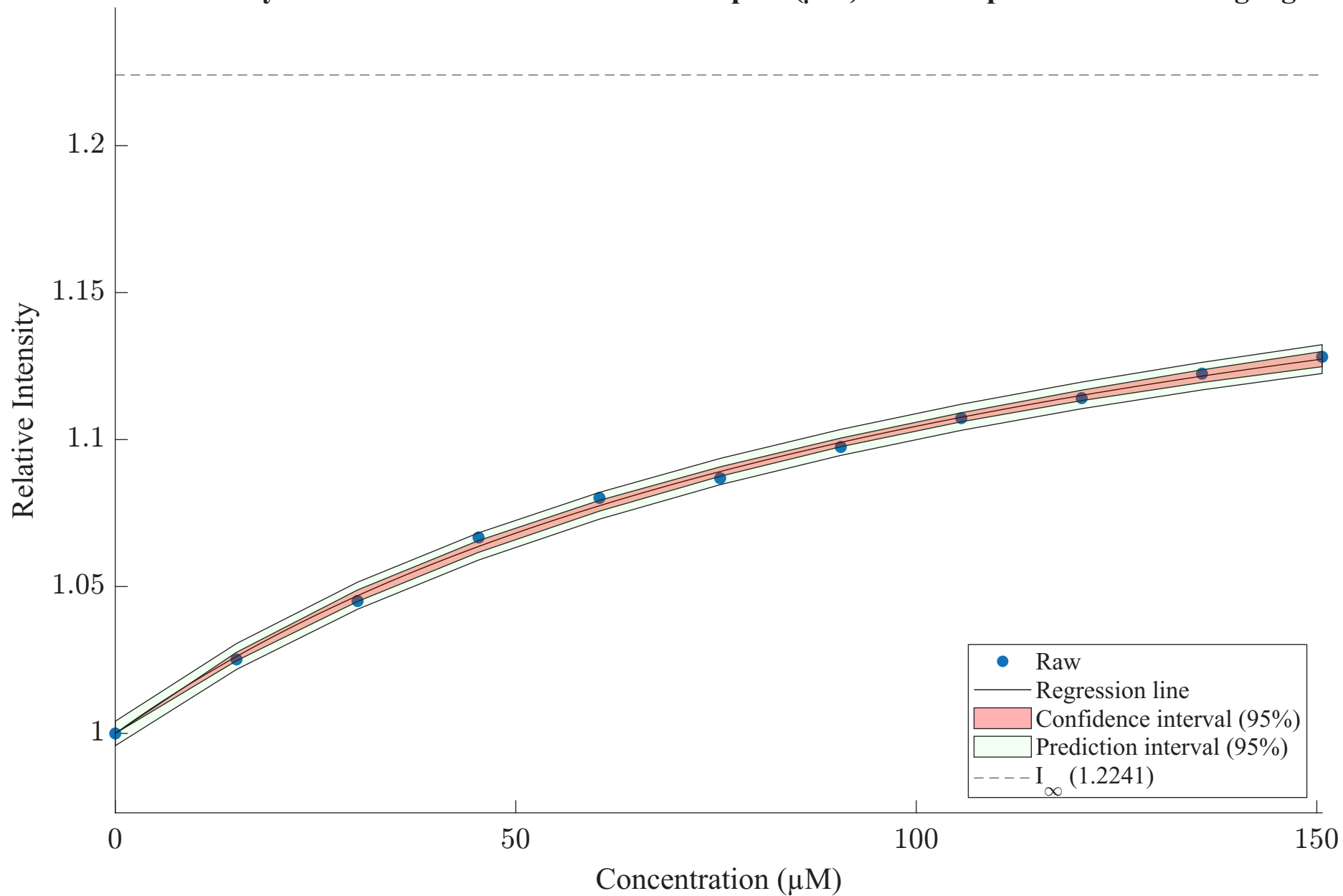
Relative intensity as a function of concentration of lipids ( \mu\text{M} ) for t1r rep2 - Statistics fitting algorithm
